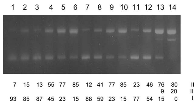
Figure 4. Cleavage of supercoiled pSP64 DNA by deglycoBLM analogues 1a and 1b . Lane 1: DNA alone; lane 2: 1.5 \mu\text{M} \text{Fe}^{2+} ; lane 3: 5 \mu\text{M} 1b ; lane 4: 1 \mu\text{M} 1b + 1.5 \mu\text{M} \text{Fe}^{2+} ; lane 5: 3 \mu\text{M} 1b + 1.5 \mu\text{M} \text{Fe}^{2+} ; lane 6: 5 \mu\text{M} 1b + 1.5 \mu\text{M} \text{Fe}^{2+} ; lane 7: 5 \mu\text{M} 1a ; lane 8: 1 \mu\text{M} 1a + 1.5 \mu\text{M} \text{Fe}^{2+} ; lane 9: 3 \mu\text{M} 1a + 1.5 \mu\text{M} \text{Fe}^{2+} ; lane 10: 5 \mu\text{M} 1a + 1.5 \mu\text{M} \text{Fe}^{2+} ; lane 11: 5 \mu\text{M} deglycoBLM \text{A}_5 ; lane 12: 1 \mu\text{M} dgBLM \text{A}_5 + 1.5 \mu\text{M} \text{Fe}^{2+} ; lane 13: 3 \mu\text{M} deglycoBLM \text{A}_5 + 1.5 \mu\text{M} \text{Fe}^{2+} ; lane 14: 5 \mu\text{M} deglycoBLM \text{A}_5 + 1.5 \mu\text{M} \text{Fe}^{2+} .
