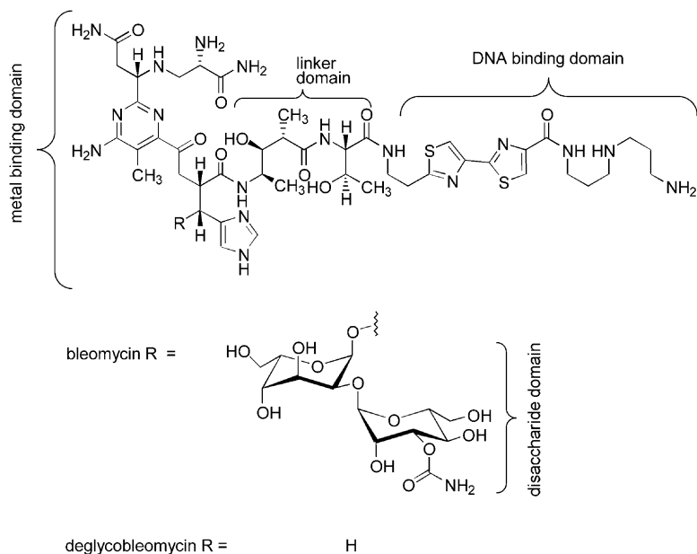
Figure 1. Structures and domains of BLM A 5 and deglycoBLM A 5 .
