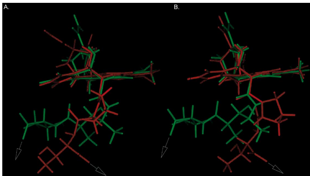
Figure 3. Comparison of Zn(II)-deglycoBLM (green) with (A) Zn(II)-deglycoBLM derivative 1a (red) and (B) Zn(II)-deglycoBLM derivative 1b (red). The DNA binding domains (arrows) have been removed for clarity.
