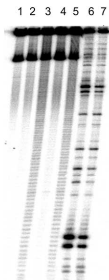
Figure 5. Cleavage of a 5'- ^{32}\text{P} end labeled DNA duplex by deglycoBLM analogues 1a and 1b . Lane 1: DNA alone; lane 2: 1 \mu\text{M} 1b + 10 \mu\text{M} \text{Fe}^{2+} ; lane 3: 10 \mu\text{M} 1b + 10 \mu\text{M} \text{Fe}^{2+} ; lane 4: 1 \mu\text{M} 1a + 10 \mu\text{M} \text{Fe}^{2+} ; lane 5: 10 \mu\text{M} 1a + 10 \mu\text{M} \text{Fe}^{2+} ; lane 6: 1 \mu\text{M} deglycoBLM \text{A}_5 + 10 \mu\text{M} \text{Fe}^{2+} ; lane 7: 10 \mu\text{M} deglycoBLM \text{A}_5 + 10 \mu\text{M} \text{Fe}^{2+} . The band of intermediate mobility in lanes 1–5 was due to adventitious non-denatured DNA.
