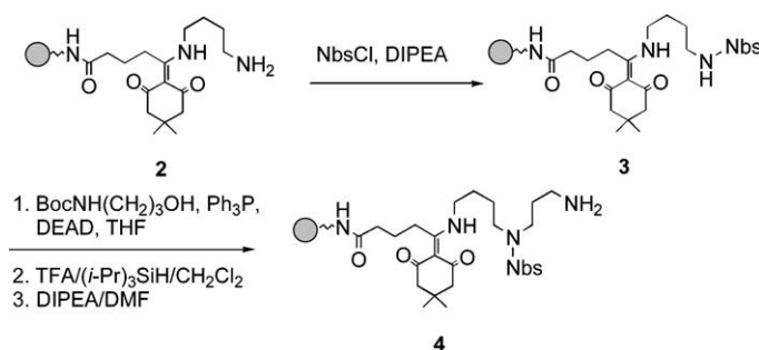
Scheme 1. Synthesis of mono-protected spermidine linked to a TentaGel resin.
