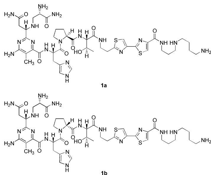
Figure 2. DeglycoBLM analogues containing S -proline ( 1a ) and R -proline ( 1b ) in place of the methylvalerate moiety.
